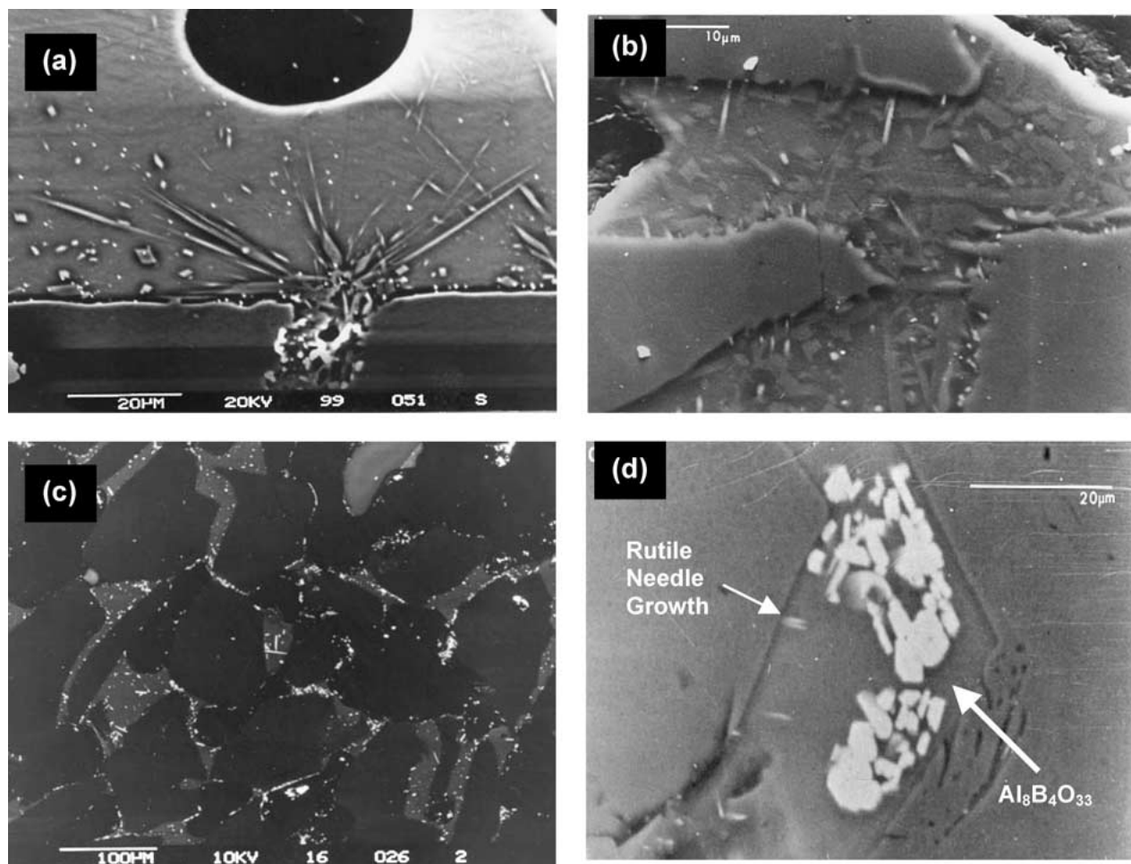
Figure 12 (a) Titania ( \text{TiO}_2 ), in the form of rutile needles, on the surface of the vitrified glass bond, (b) vitrified glass bond etched with 40% HF in water to show rutile formation within the glass bonding system, (c) electron backscattered image showing needle growth into the glass bond from the abrasive, and (d) de-vitrified glass bond containing crystals of \text{Al}_{18}\text{B}_4\text{O}_{33} bounded by two abrasive grains.
