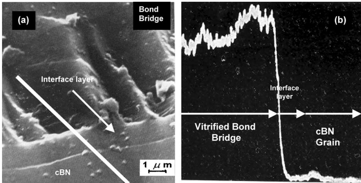
Figure 15 (a) Polished cross section of cBN abrasive and bond bridge clearly showing the interface layer, (b) electron probe microanalysis of oxygen across the line scan shown in (a), left-to-right.
