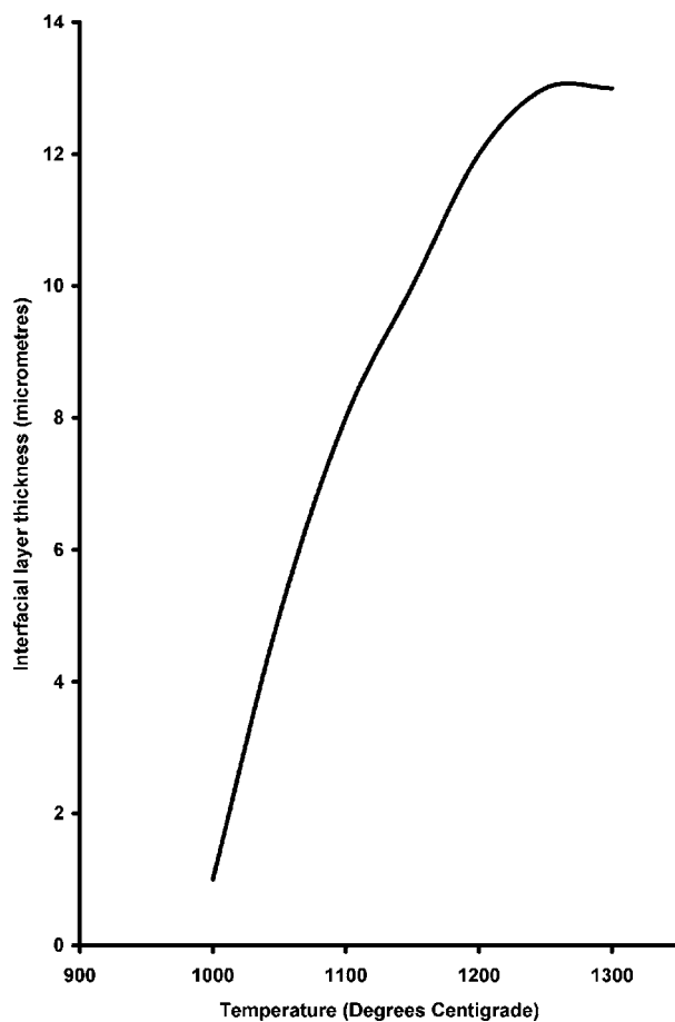
Figure 16 Interfacial layer thickness between cBN and vitrified bonding bridge as a function of sintering temperature.
