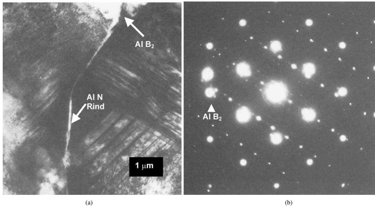
Figure 6 (a) Two contacting cBN grains separated at intervals by an AlN rind which is parallel to the cBN [110] planes. The outer edges of the grains are in contact with a featureless AlB 2 layer, (b) Selected area diffraction pattern from part of the field of contact showing the relative orientation of phases present. The smaller spots are AlN, and the larger spots are cBN. The arrow indicates the single spot generated by AlB 2 phase.
