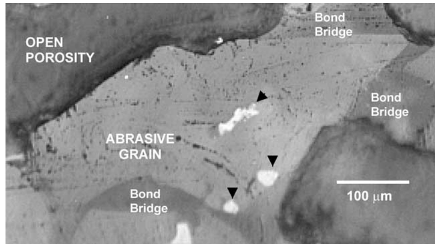
Figure 4 High purity aluminium oxide grinding wheel showing enriched regions of \text{Na}_2\text{O} determined using an electron probe micro analyzer.
