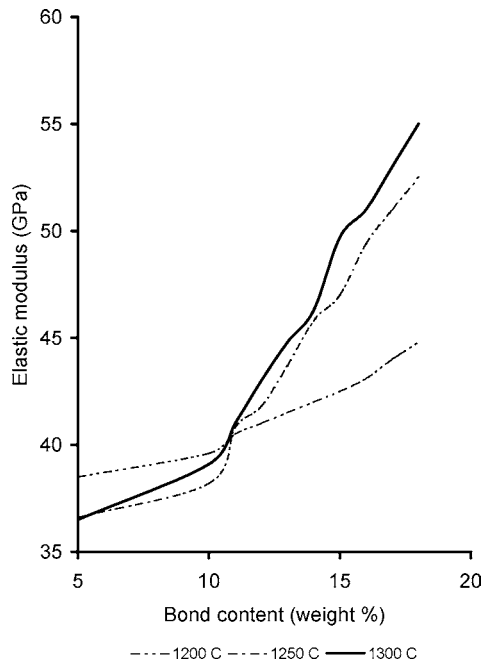
Figure 9 Effect of bond content and firing temperature on the elastic modulus of high purity aluminium oxide structures.
