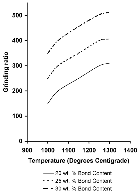
Figure 13 Relationship between grinding ratio and firing temperature as a function of bond content for vitrified cBN grinding wheel structures.
