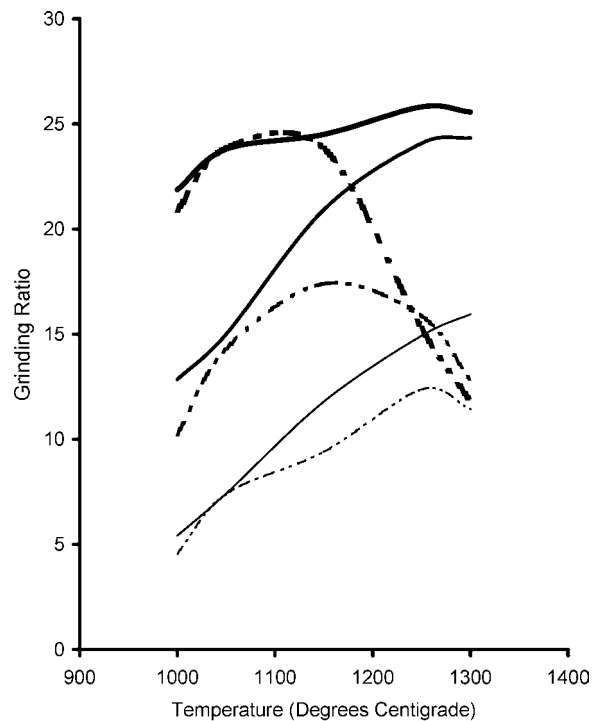
— High purity corundum plus 5 wt.% bond --- Titanium-doped corundum plus 5 wt.% bond — High purity corundum plus 12 wt.% bond - · - Titanium-doped corundum plus 12 wt.% bond — High purity corundum plus 19 wt.% bond - · - Titanium-doped corundum plus 19 wt.% bond
