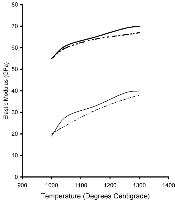
--- Titanium-doped corundum plus 5wt.% bond and 45wt.% porosity — High purity corundum plus 5wt.% bond and 45wt.% porosity - · - Titanium-doped corundum plus 19wt.% bond and 26 wt.% porosity — High purity corundum plus 19wt.% bond and 36wt.% porosity
