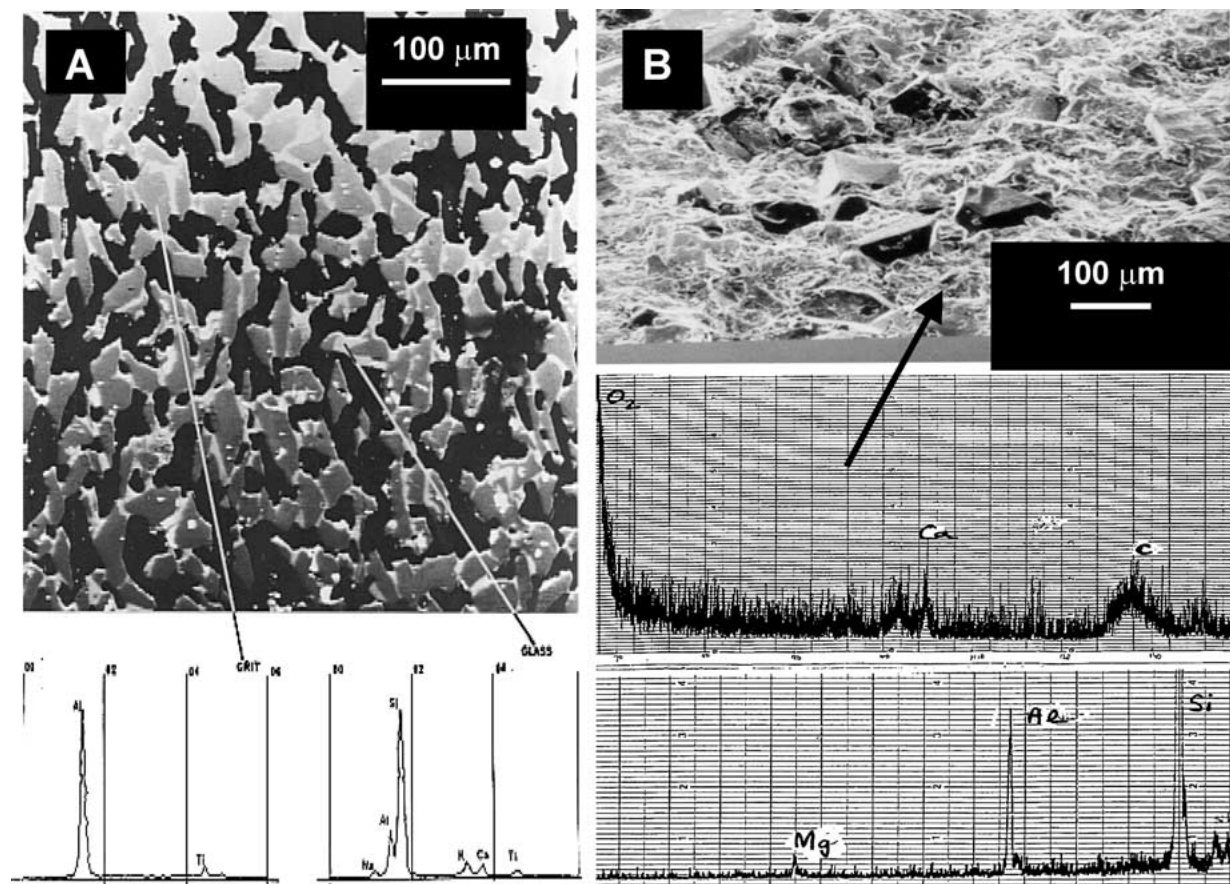
Figure 7 Electron probe microanalysis of (A) titanium-doped aluminium oxide and vitrified glass bonding system and (B) cBN and vitrified glass bonding system.
