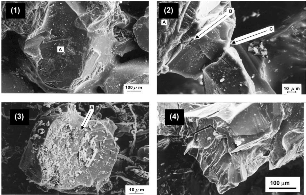
Figure 3 Grinding wheel wear mechanisms: (1) abrasive wear showing (A) wear flat on the tip of the grain; (2) bonding bridge fracture showing (A) abrasive grain, (B) interfacial layer, and (c) bond bridge; (3) abrasive grain fracture showing (A) grain fracture through the (0001) basal plane; and (4) interface fracture between abrasive grain and bond bridge.
