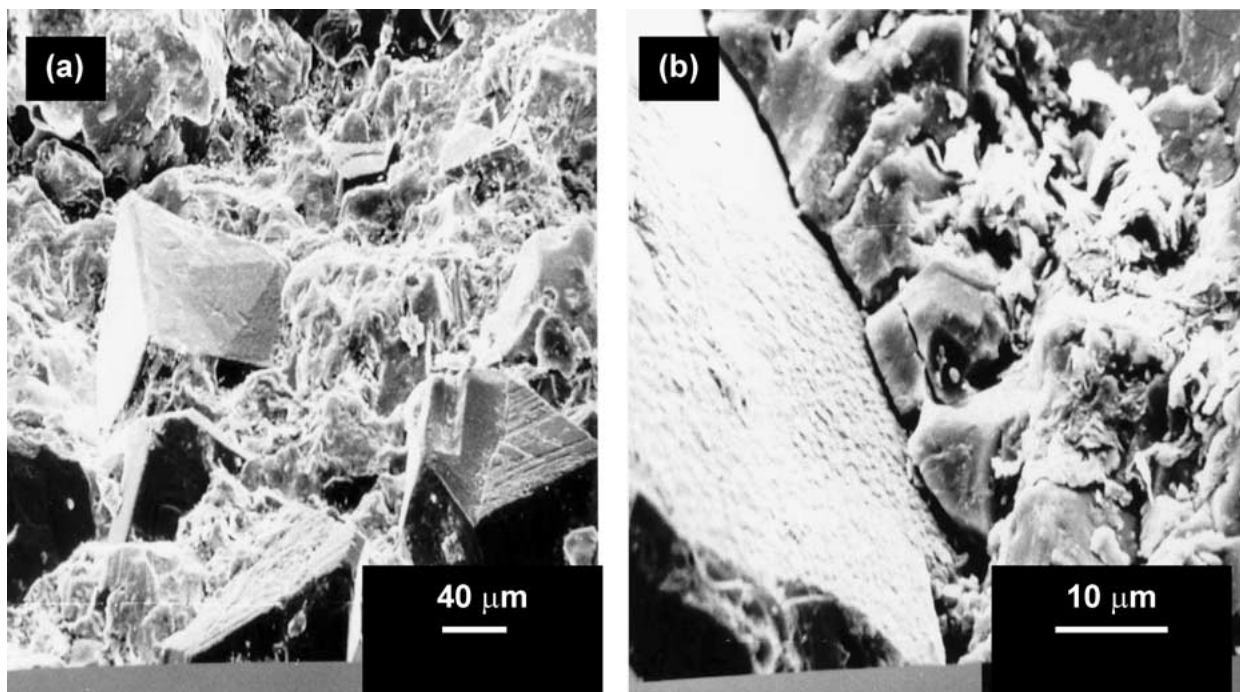
Figure 14 (a) Vitrified cBN grinding wheel structure and (b) interface between cBN abrasive grain and vitrified bonding.
